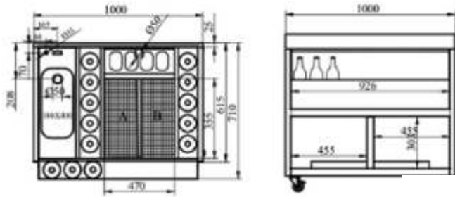
MODS001 SINK COMPACT Modulo Cocktail Station Inox Aisi304 18/10 – 100*70*83h cm
