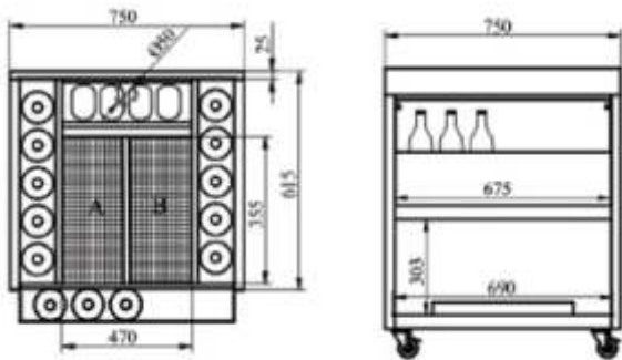
MODI001 COMPACT Modulo Cocktail Station Inox Aisi304 18/10 – 75*70*83h cm
